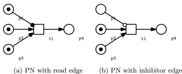
Fig. 9: Additional types of edges
