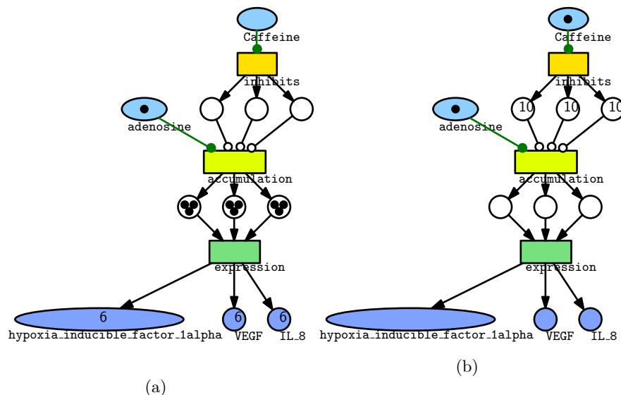
Fig. 15: Animated Petri net (a) Initial marking: 1 token in adenosine. Step count: 10 (b) Initial marking: 1 token in Caffeine and 1 token in adenosine. Step count: 10
