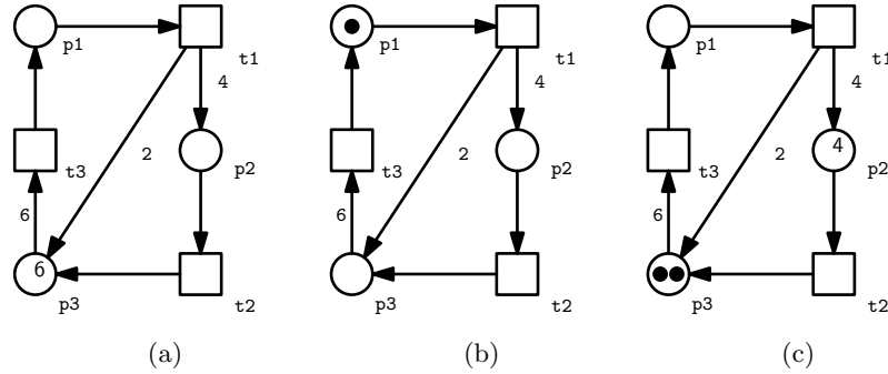
Fig. 8: Firing rule
