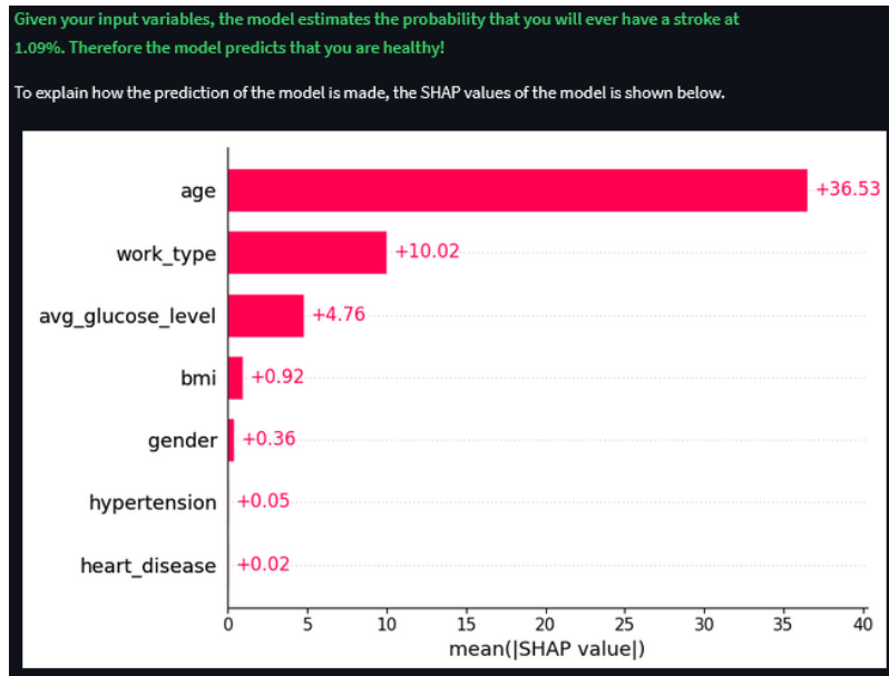
Figure 9: A stroke prediction of a logistic regression attached with SHAP values
